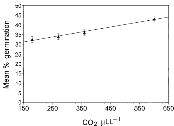
Fig. 1 Mean percentage of seeds germinated by 30 days at 180, 270, 360, and 600 \mu\text{L L}^{-1} CO 2 concentrations. Error bars represent one standard error. P = 0.006 from logistic regression analysis of germination of individual seeds.
