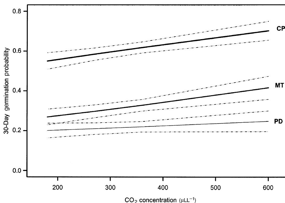
Fig. 3 Logistic regression fits (solid lines) and 95% confidence intervals (dashed lines) of the probability of germinating by 30 days as a function of CO 2 and Region of origin. Seeds collected from Coastal Plain ('CP') and Mountain ('MT') regions exhibit a positive effect of CO 2 on germination probability ( P < 0.0001 and P = 0.0002 , respectively), while seeds from the Piedmont ('PD') show no overall response to atmospheric CO 2 .
