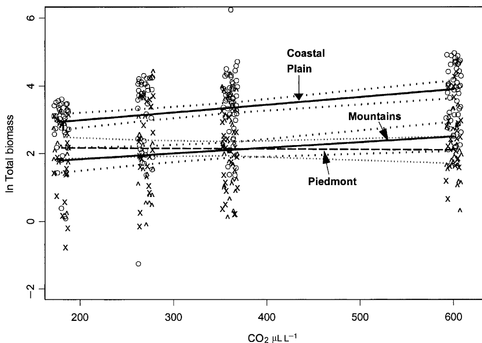
Fig. 5 Linear regression fits (solid lines for Coastal Plain and Mountains; dashed line for Piedmont) and 95% confidence intervals (dotted lines) for the ln-transformed total biomass of plants in each Region vs. atmospheric CO 2 . Points represent individual trees. Coastal Plain ('o') and Mountain ('x') trees exhibit increasing biomass with increasing CO 2 (CP: P < 0.001 and N = 168 , MT: P = 0.035 and N = 87 ). Piedmont trees ('^') show no effect of CO 2 on total biomass ( P = 0.8 and N = 101 ). Note that the results do not change with the exclusion of the small and large Coastal Plain trees at 270 \mu\text{L L}^{-1} and 360 \mu\text{L L}^{-1} , respectively, or the smallest Mountain tree at 180 \mu\text{L L}^{-1} .
