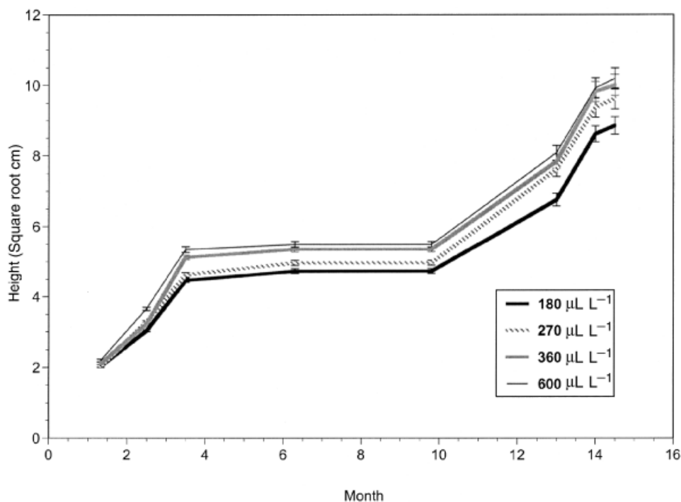
Fig. 4 CO 2 interacts significantly with Time to explain height growth in A. rubrum ( P = 0.01 from repeated-measures nested ANOVA). The mean values of square-root transformed height for each CO 2 group at each of the eight height censuses are shown. Error bars represent \pm 1 SE. Note that the dormant measurements (months = 6.3 and 9.8) were not included in the analysis.
