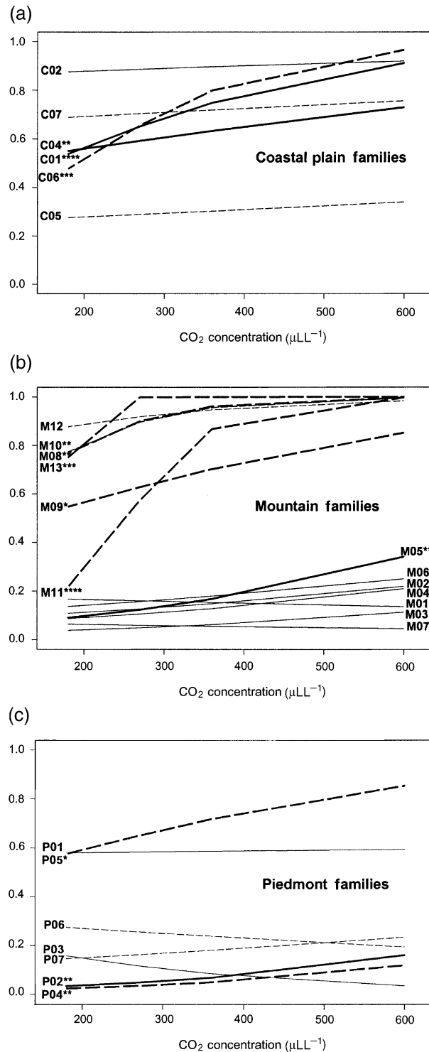
Fig. 2 (a–c) Logistic regression fits of the probability of germinating within 30 days ( y -axis) as a function of atmospheric CO 2 carried out separately for each family originating from the (a) Coastal Plain (C01–C07), (b) Mountains (M01–M13), and (c) Piedmont (P01–P07). Dark lines depict families exhibiting significant responses to CO 2 ; pale lines denote no significant response. For each region, solid lines represent fits for families from Population 1, and dashed lines denote families from Population 2. *Refers to CO 2 parameters in logistic regressions having P < 0.10 , **signifies P < 0.05 , ***refers to P < 0.01 , and ****denotes P < 0.001 . Lack of asterisks indicates that there was no significant germination response to CO 2 .
